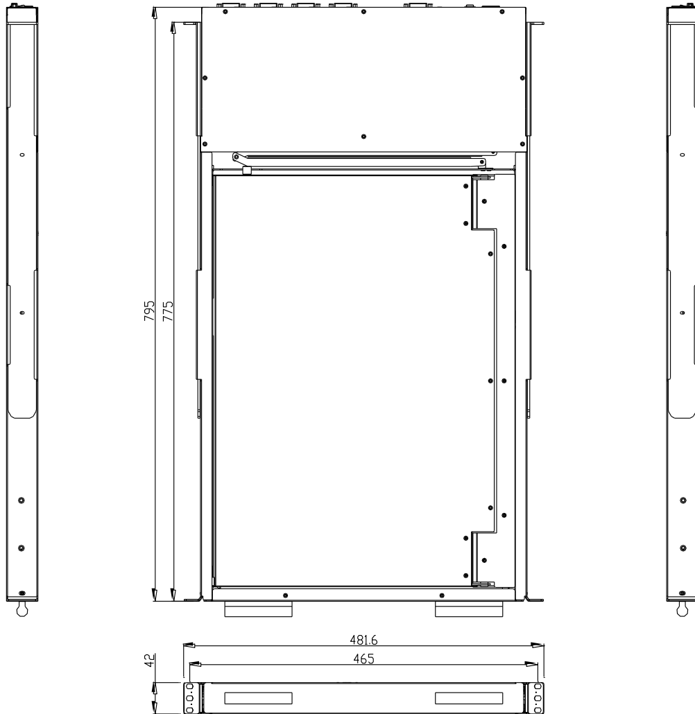
Rear of KVM-2104/2404QSS-M2
